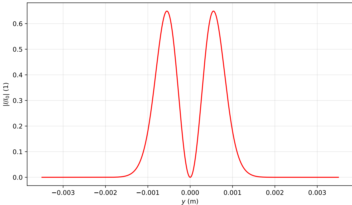
Intensity profile I(x=0, y, z=0.876)/I_0 , P_{in}=0.5P_{cr} , artificial time
